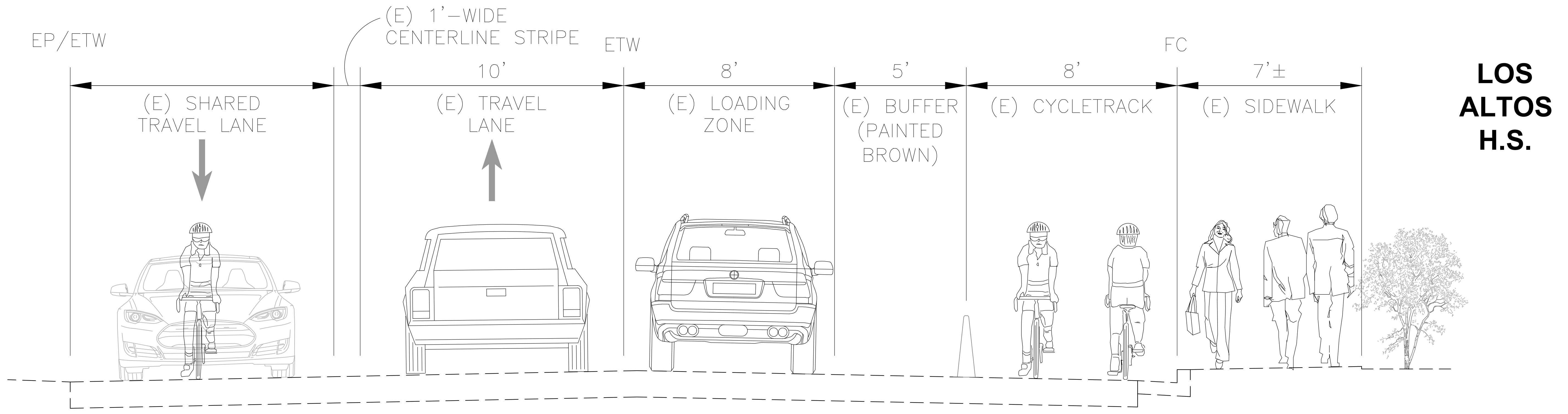
EXISTING CROSS SECTION - FACING EAST JARDIN DRIVE SCALE: NOT TO SCALE
