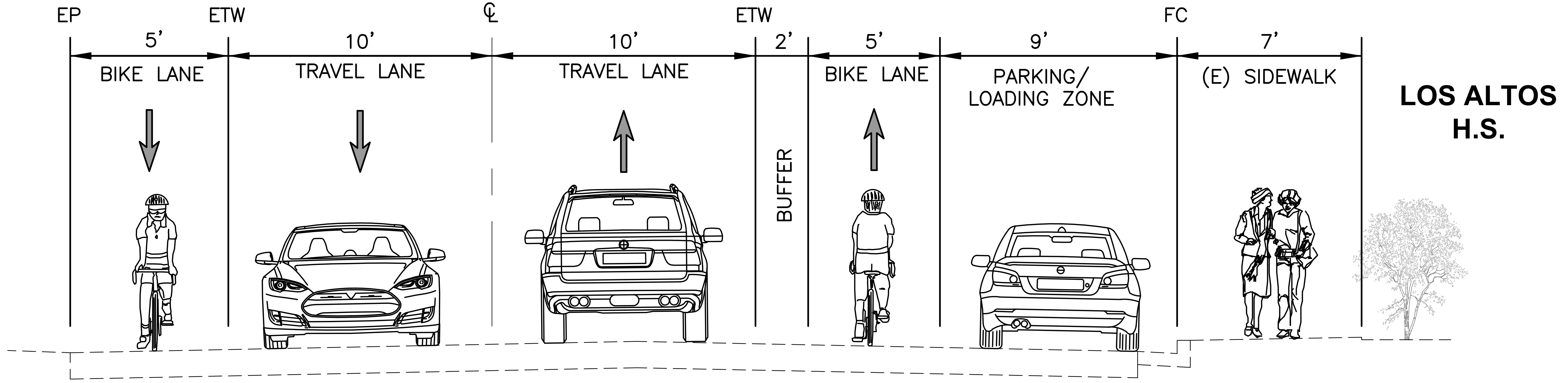
RECOMMENDED PLAN JARDIN DRIVE PROPOSED CROSS SECTION - FACING EAST (VALENCIA DRIVE TO ALICIA WAY) SCALE: NOT TO SCALE
