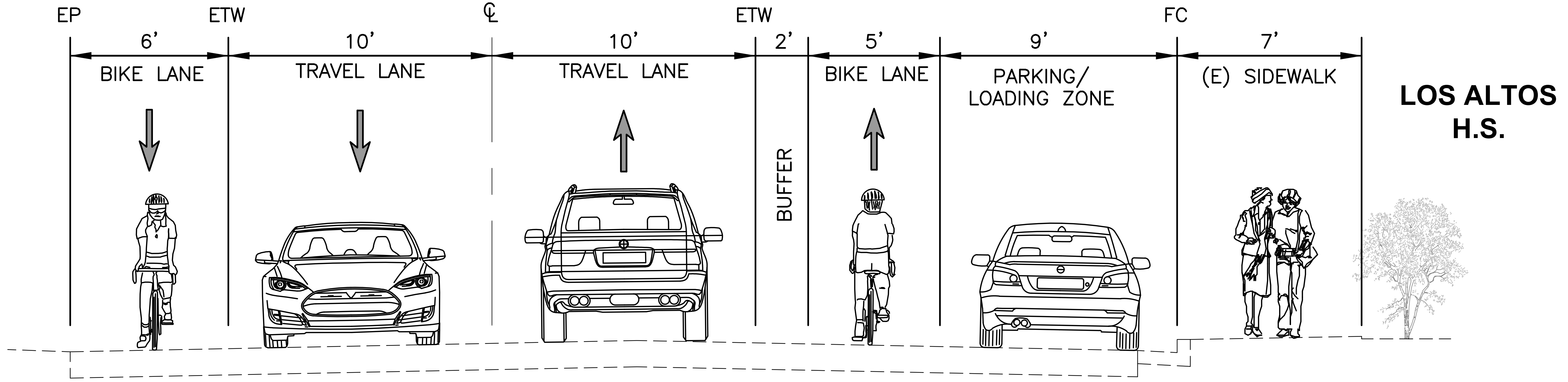
RECOMMENDED PLAN JARDIN DRIVE PROPOSED CROSS SECTION - FACING EAST (VALENCIA DRIVE TO ALICIA WAY)
