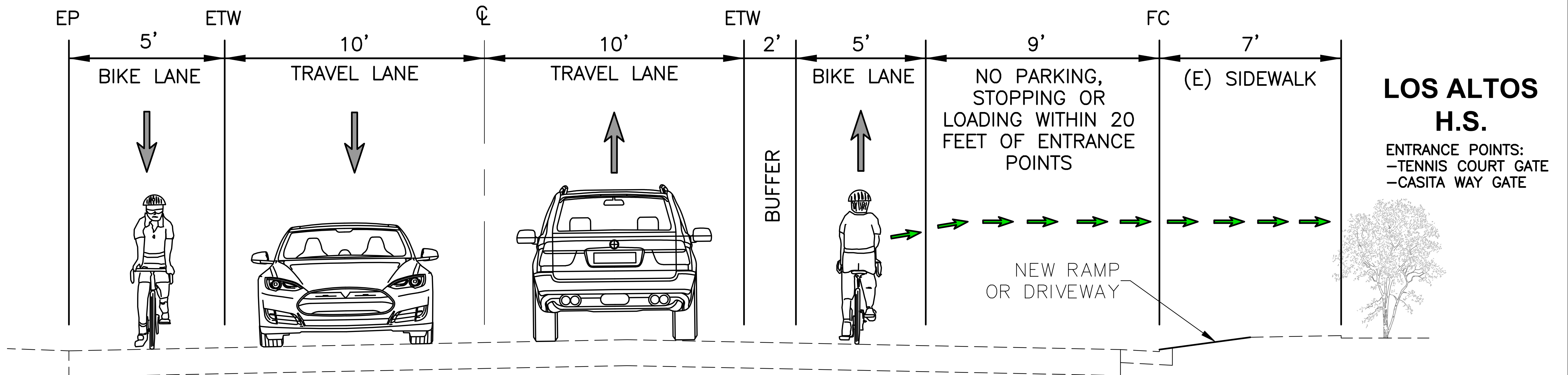
RECOMMENDED PLAN JARDIN DRIVE PROPOSED CROSS SECTION - FACING EAST AT STUDENT ENTRANCE POINTS TO HIGH SCHOOL
