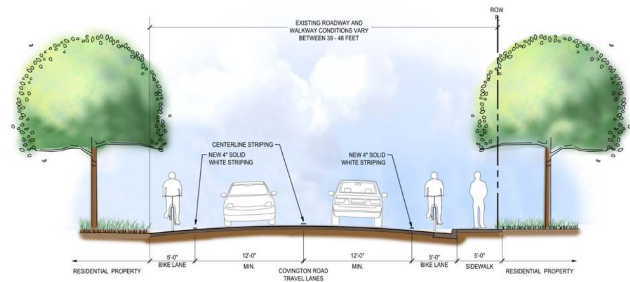
3 TYPICAL ROADWAY SECTION (PROPOSED) 1"=5'-0"
