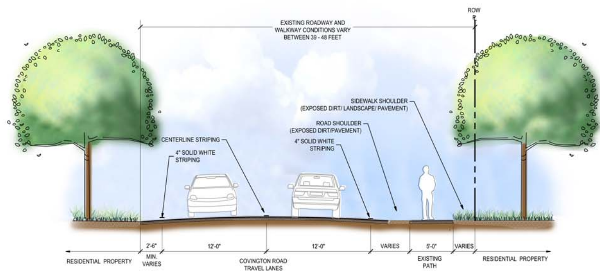
2 TYPICAL ROADWAY SECTION (EXISTING) 1"=5'-0"
